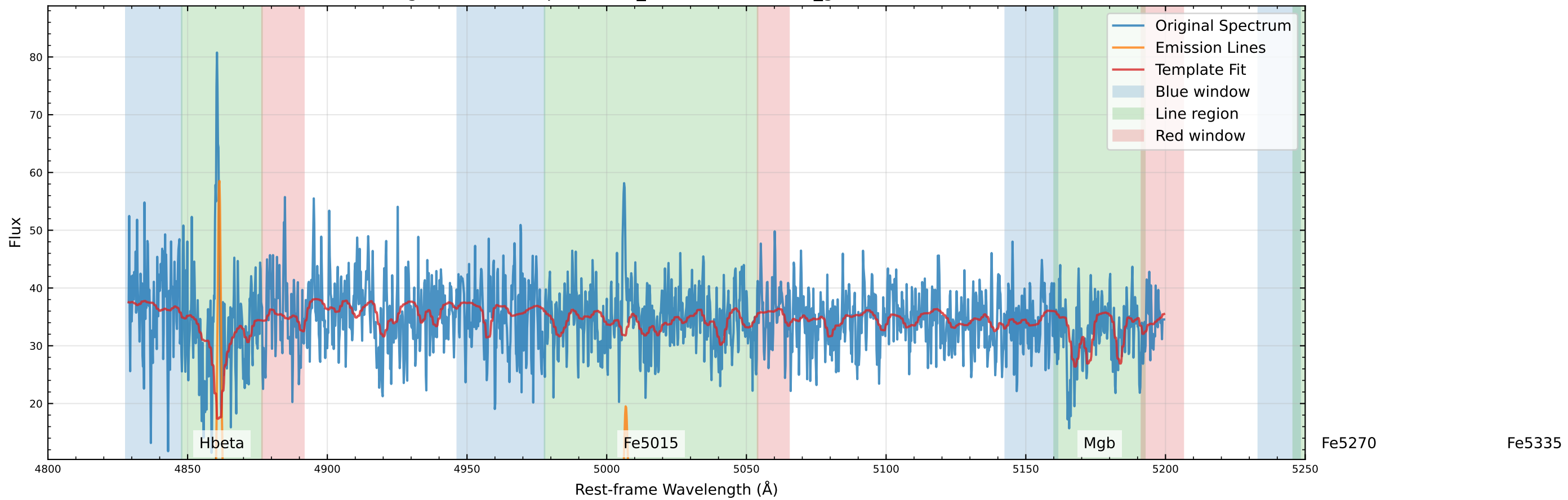
Original Data Comparison (v_star=-70.6 km/s, v_gas=-49.1 km/s)
