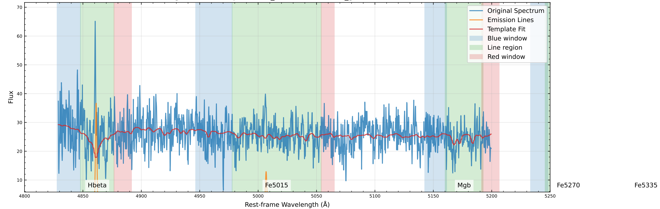
Original Data Comparison (v_star=-43.5 km/s, v_gas=-51.4 km/s)
