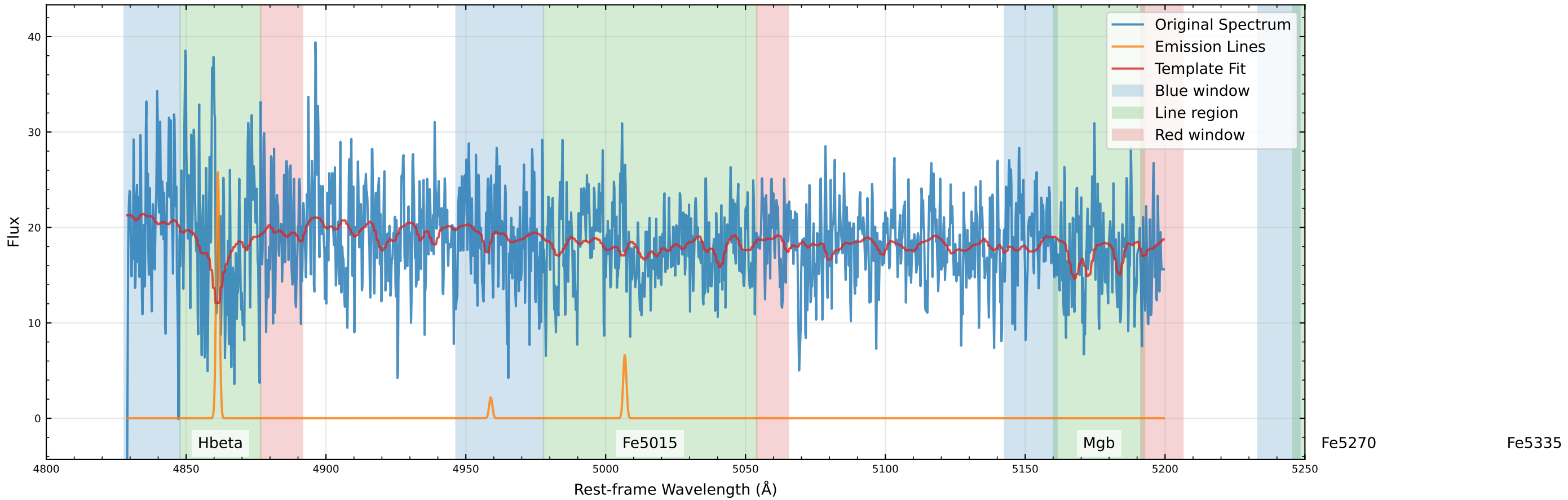
Original Data Comparison (v_star=-101.2 km/s, v_gas=-98.6 km/s)
