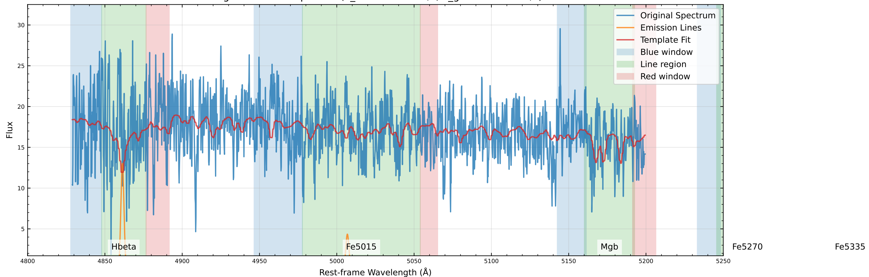
Original Data Comparison (v_star=-87.9 km/s, v_gas=-107.7 km/s)
