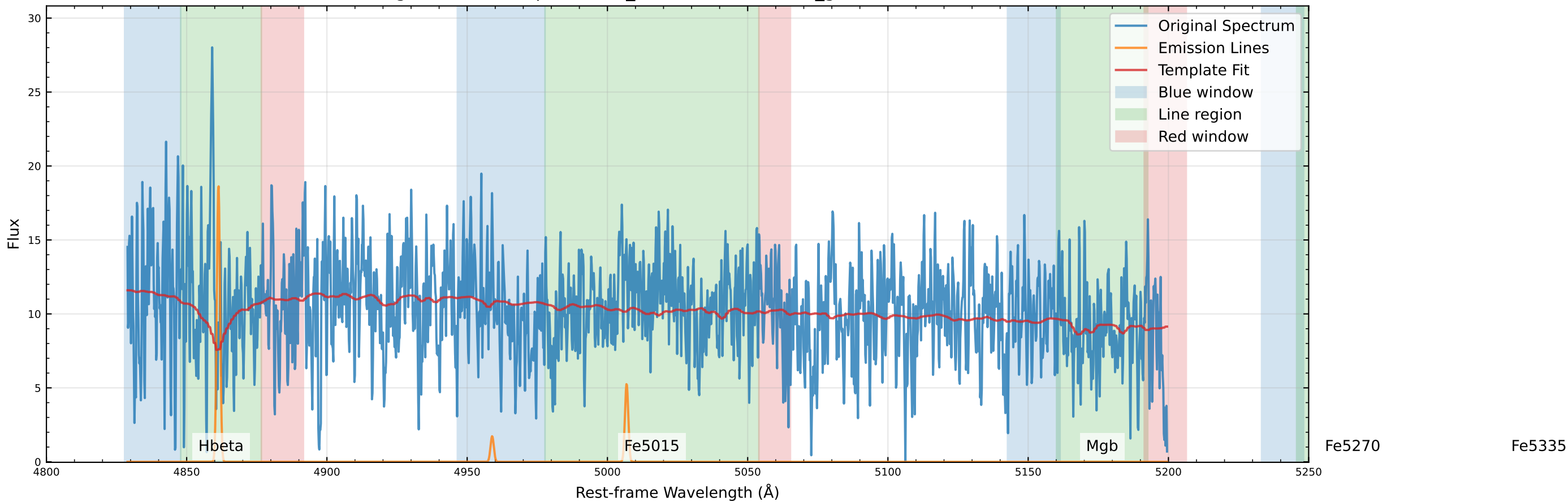
Original Data Comparison (v_star=-151.1 km/s, v_gas=-142.3 km/s)
