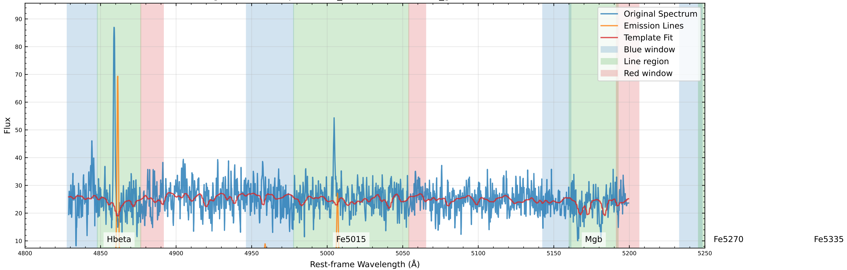
Original Data Comparison (v_star=-117.1 km/s, v_gas=-140.2 km/s)
