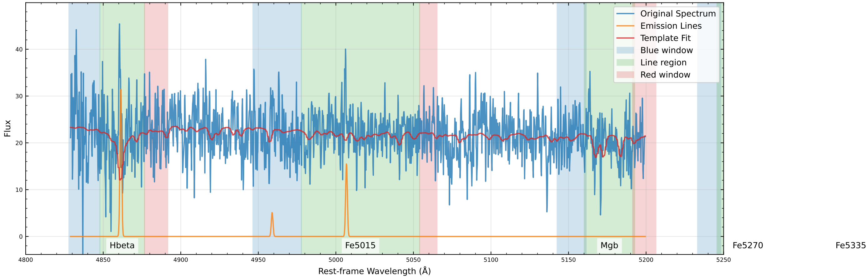
Original Data Comparison (v_star=-52.5 km/s, v_gas=-47.1 km/s)
