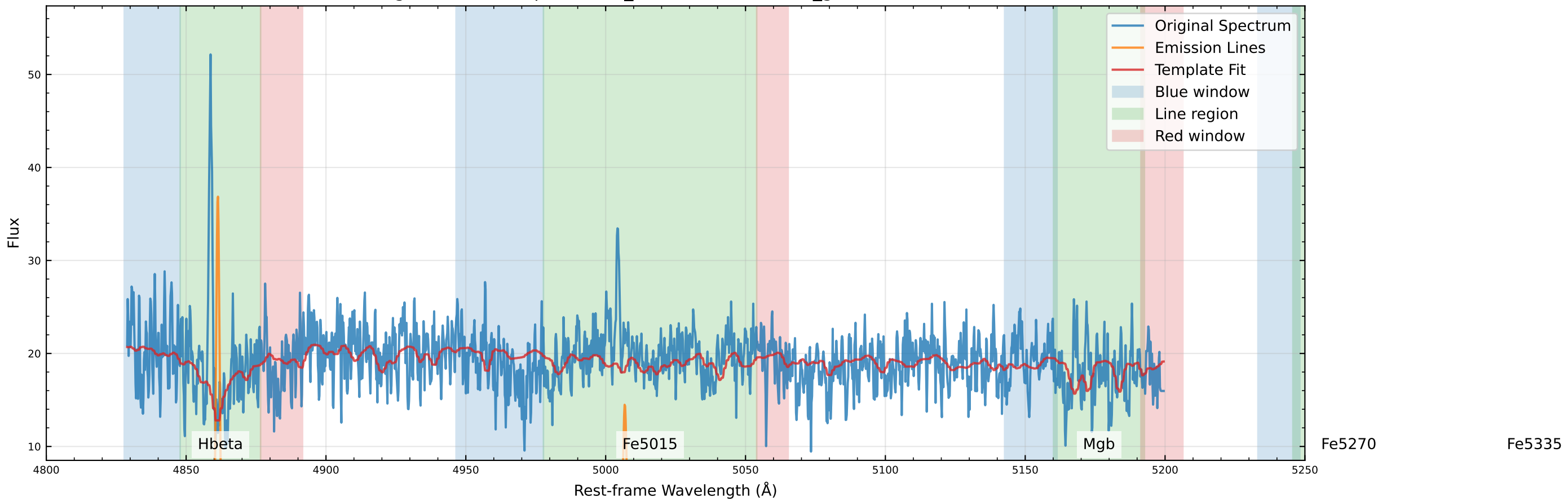
Original Data Comparison (v_star=-157.2 km/s, v_gas=-159.7 km/s)
