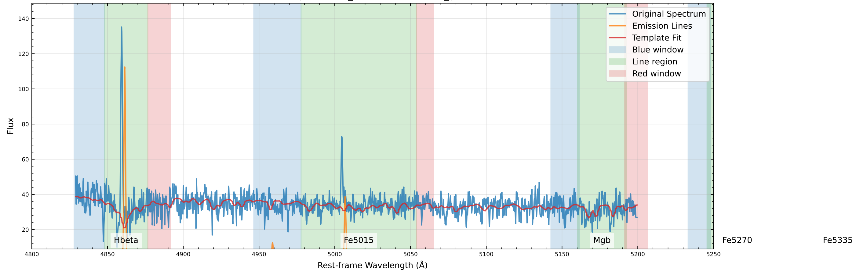
Original Data Comparison (v_star=-99.2 km/s, v_gas=-126.6 km/s)
