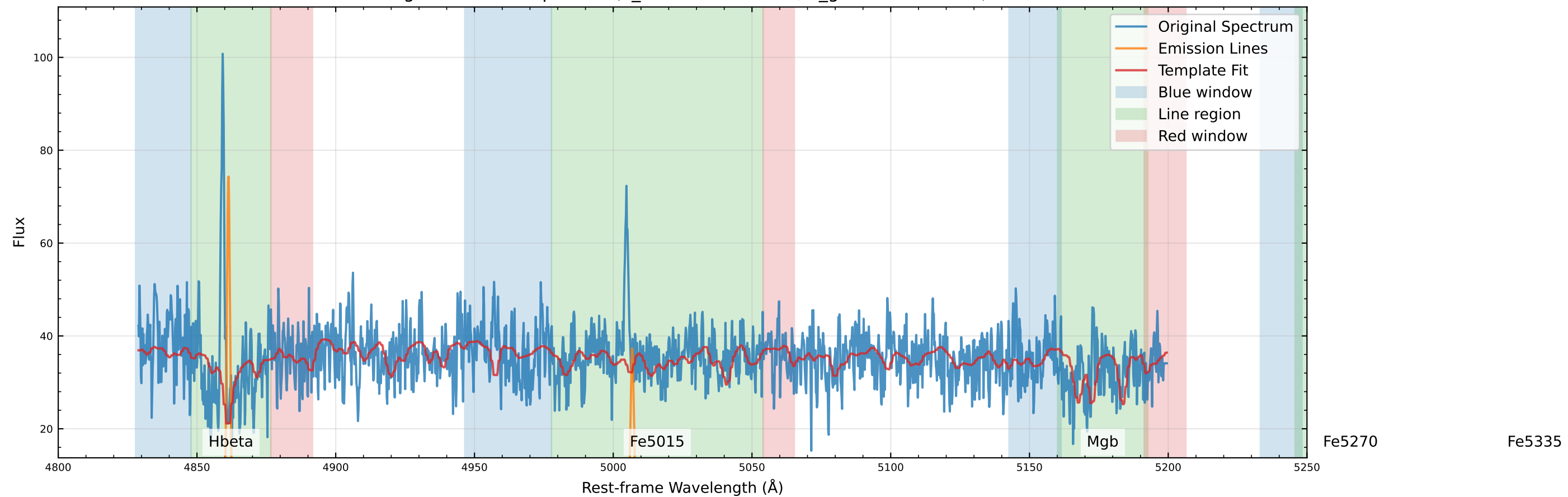
Original Data Comparison (v_star=-126.5 km/s, v_gas=-128.7 km/s)
