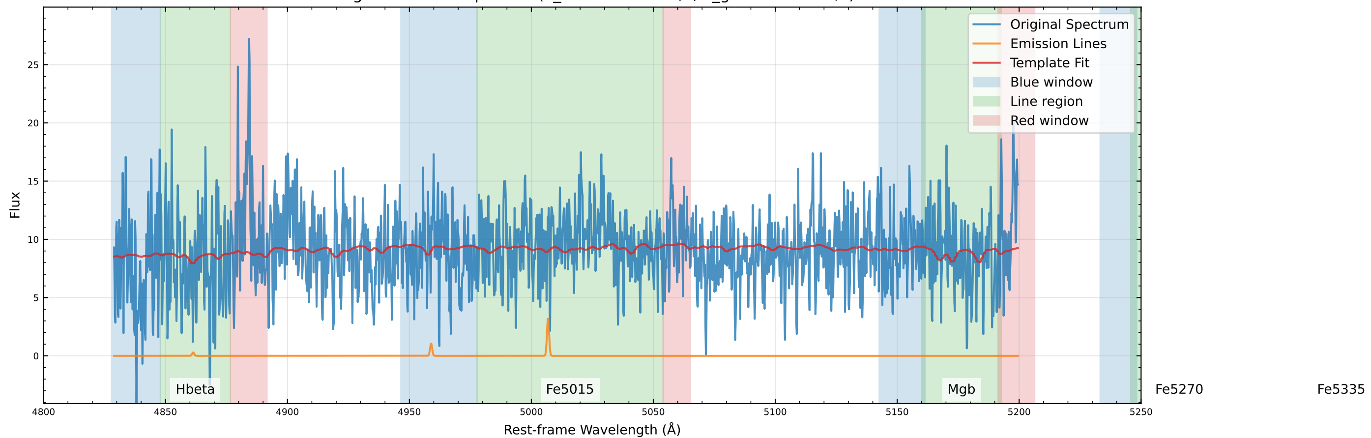
Original Data Comparison (v_star=130.1 km/s, v_gas=110.1 km/s)
