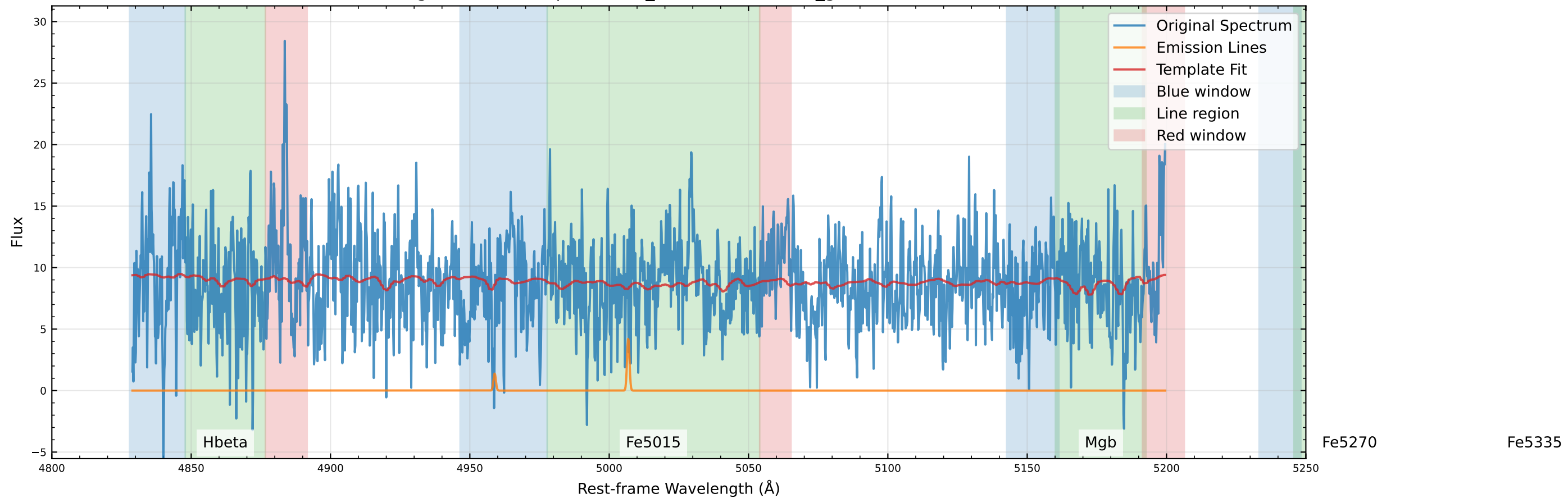
Original Data Comparison (v_star=59.8 km/s, v_gas=98.4 km/s)
