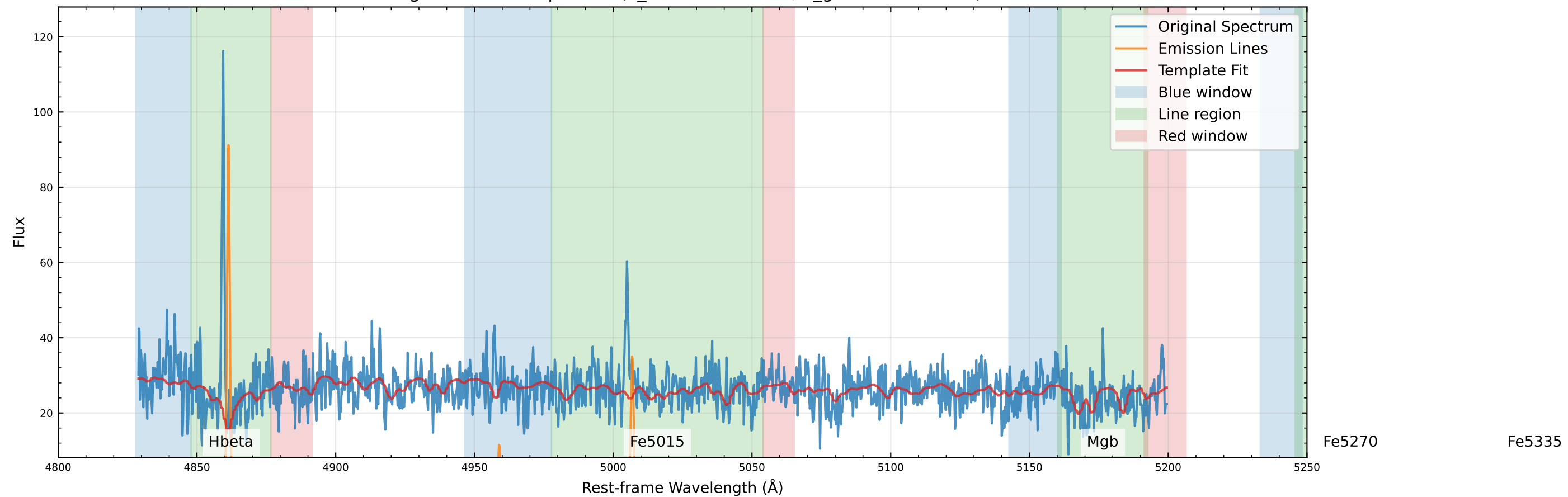
Original Data Comparison ( v_{\text{star}}=-53.5 km/s, v_{\text{gas}}=-119.3 km/s)
