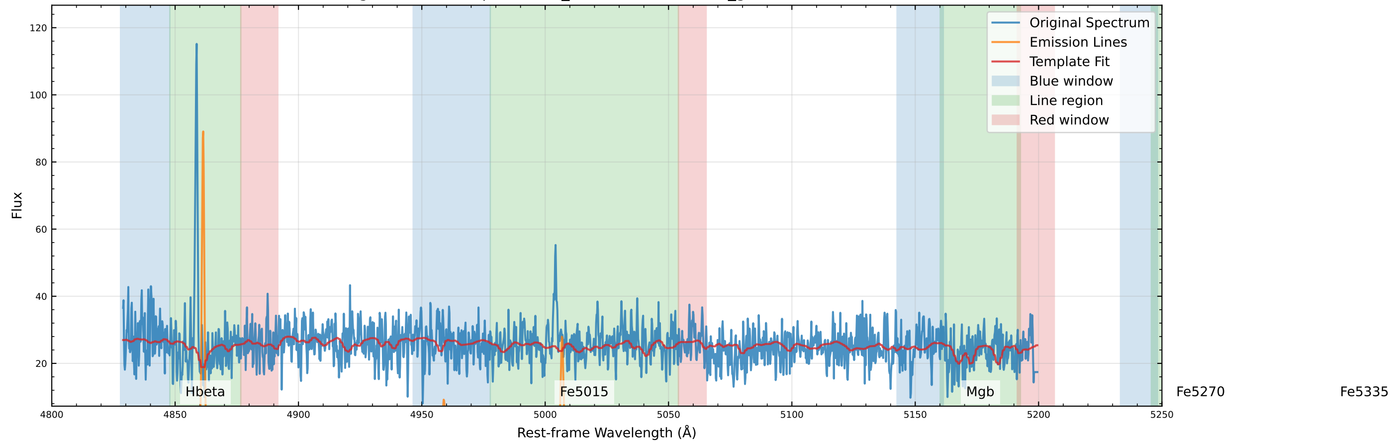
Original Data Comparison (v_star=-156.4 km/s, v_gas=-167.0 km/s)
