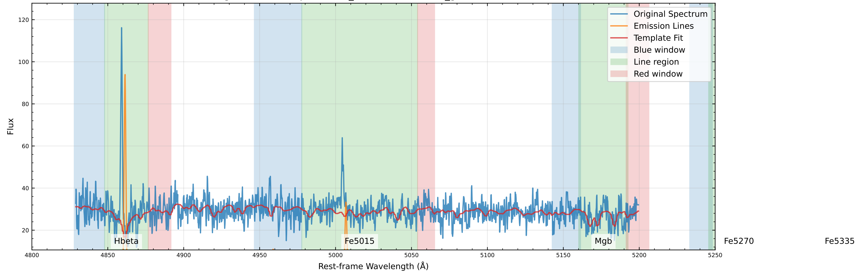
Original Data Comparison ( v_{\text{star}}=-95.6 km/s, v_{\text{gas}}=-140.8 km/s)
