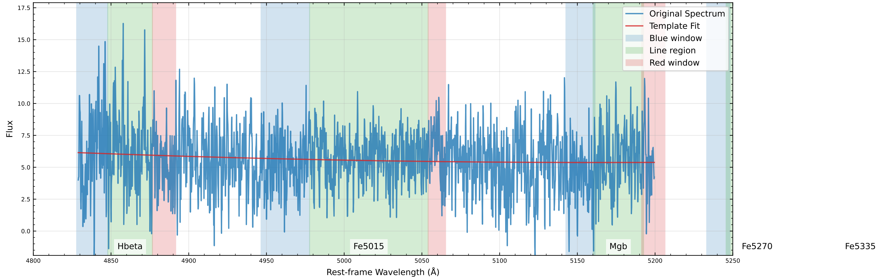
Original Data Comparison (v_star=-55.9 km/s)
