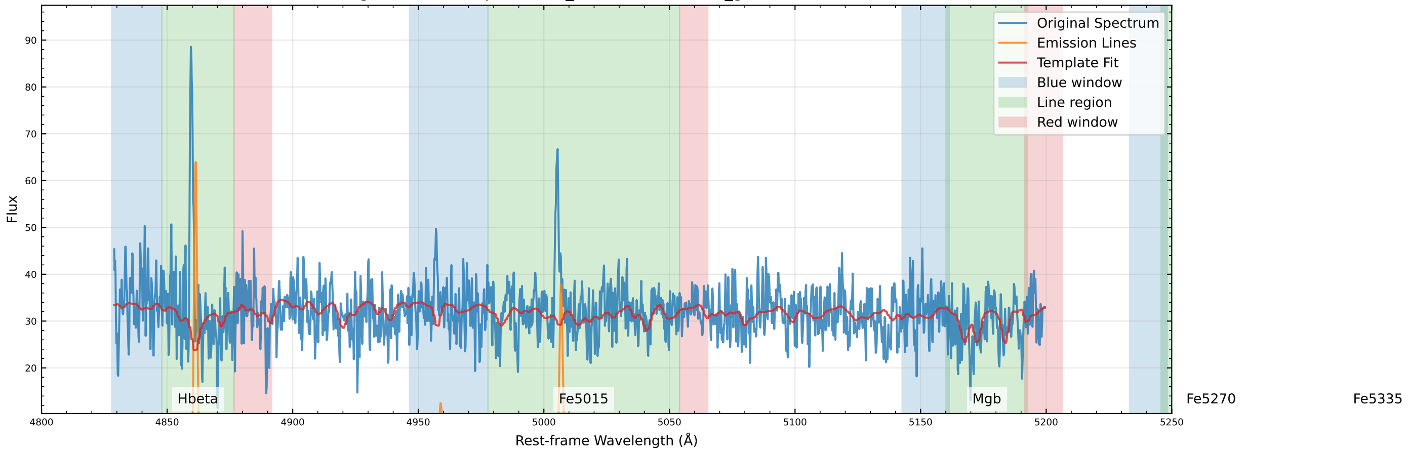
Original Data Comparison (v_star=-97.6 km/s, v_gas=-101.2 km/s)
