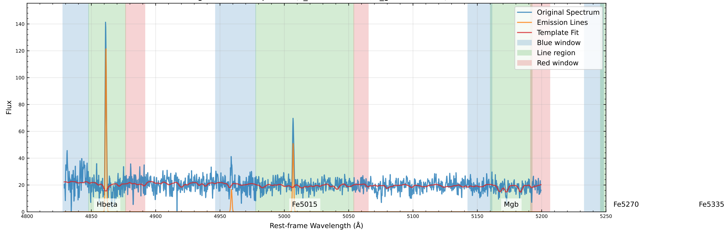
Original Data Comparison ( v_{\text{star}}=-6.1 km/s, v_{\text{gas}}=-7.5 km/s)
