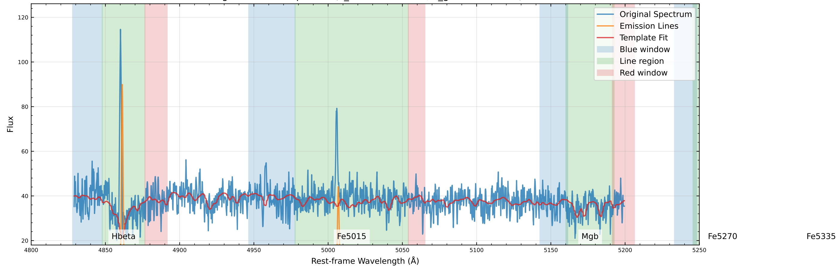
Original Data Comparison (v_star=-79.8 km/s, v_gas=-71.1 km/s)
