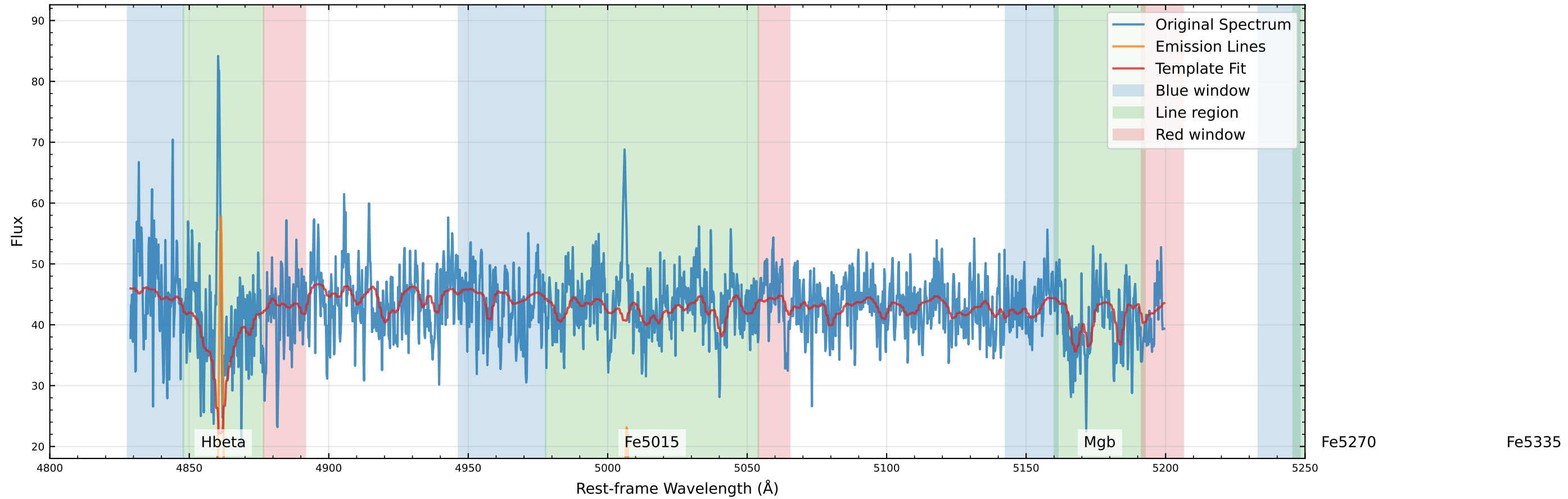
Original Data Comparison (v_star=-60.2 km/s, v_gas=-51.1 km/s)
