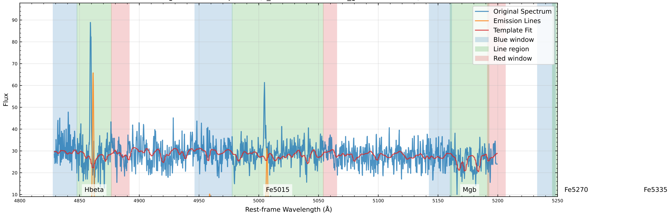
Original Data Comparison (v_star=-117.0 km/s, v_gas=-127.2 km/s)
