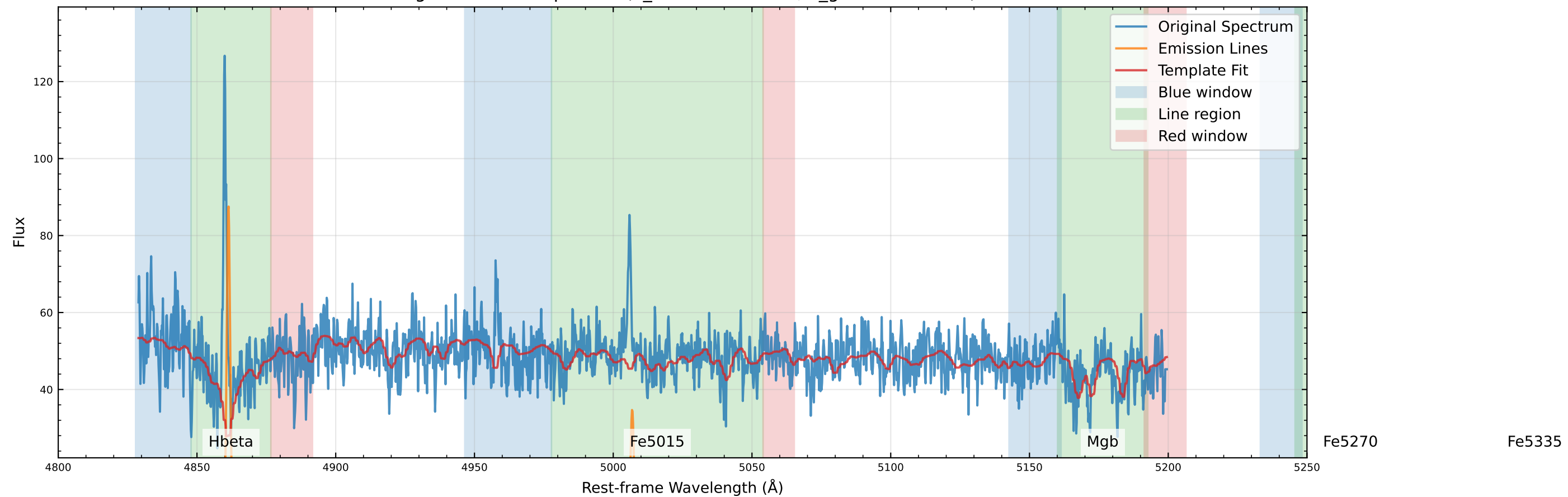
Original Data Comparison (v_star=-68.8 km/s, v_gas=-77.4 km/s)
