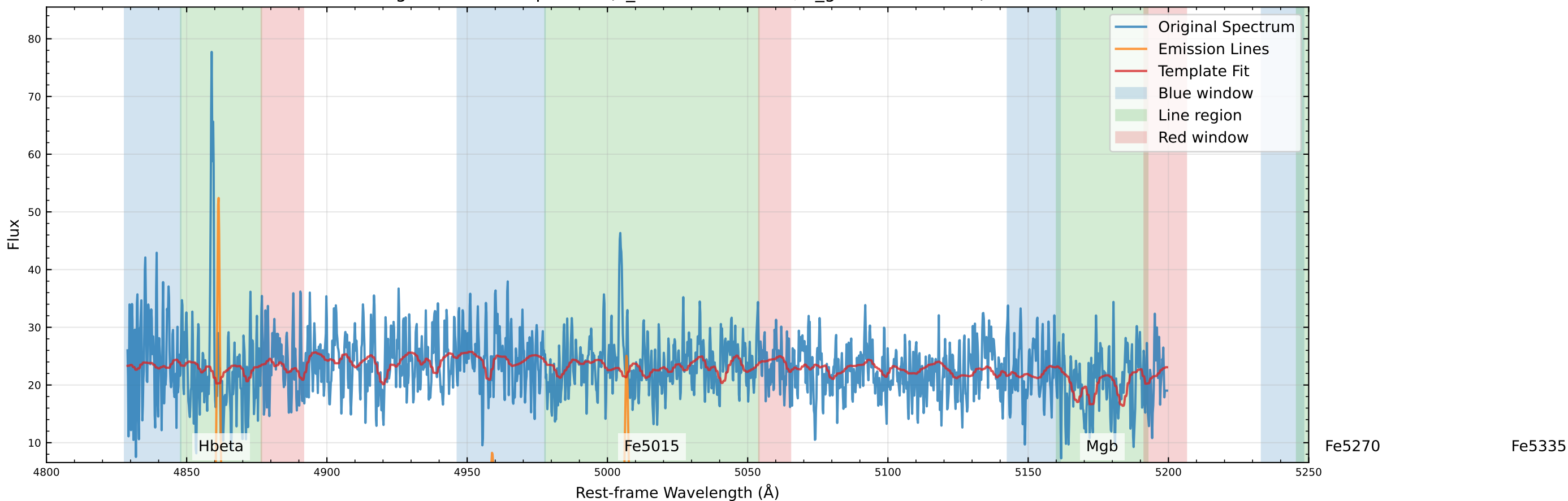
Original Data Comparison (v_star=-109.8 km/s, v_gas=-137.7 km/s)
