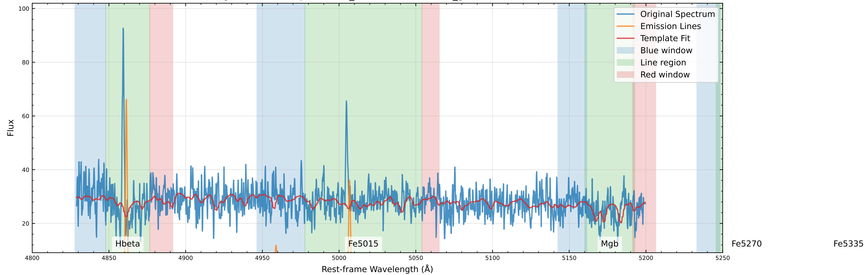
Original Data Comparison (v_star=-125.4 km/s, v_gas=-123.5 km/s)
