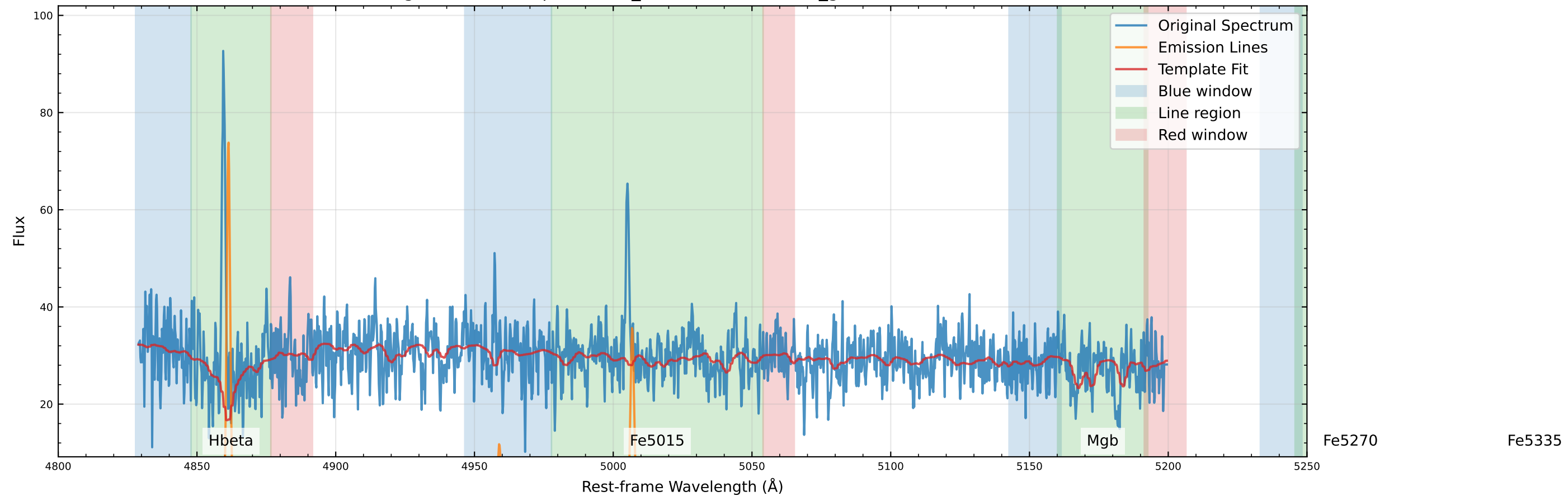
Original Data Comparison (v_star=-118.0 km/s, v_gas=-106.8 km/s)
