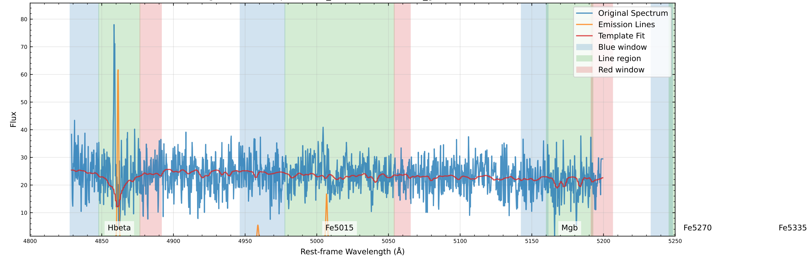
Original Data Comparison (v_star=-152.1 km/s, v_gas=-159.6 km/s)
