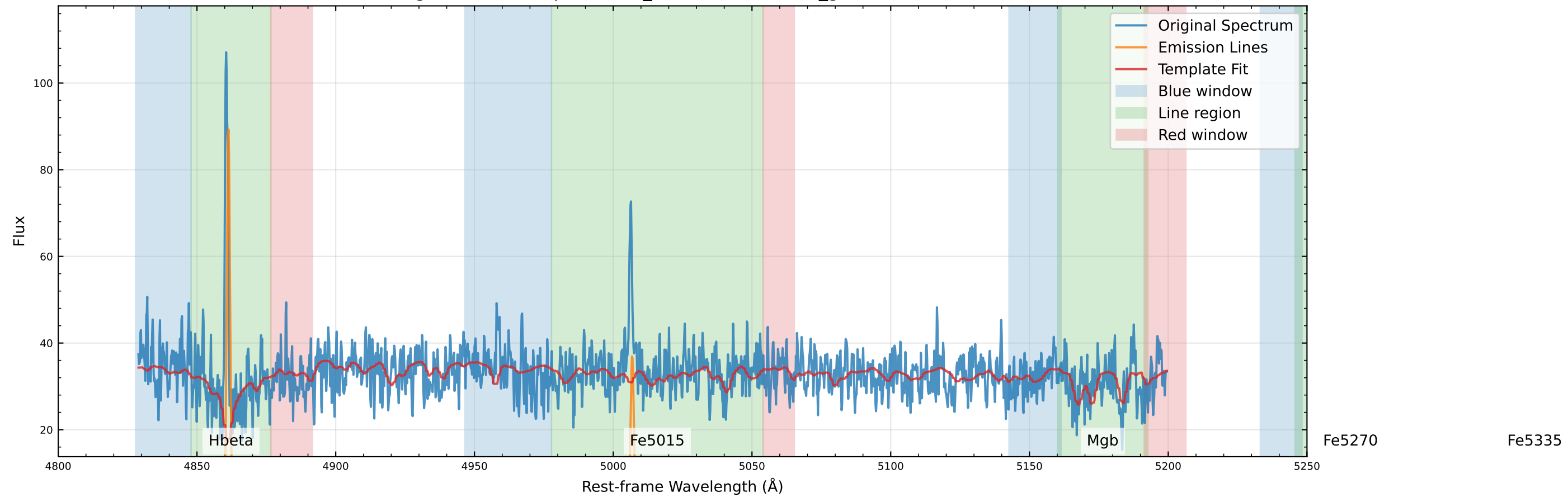
Original Data Comparison (v_star=-58.8 km/s, v_gas=-41.4 km/s)
