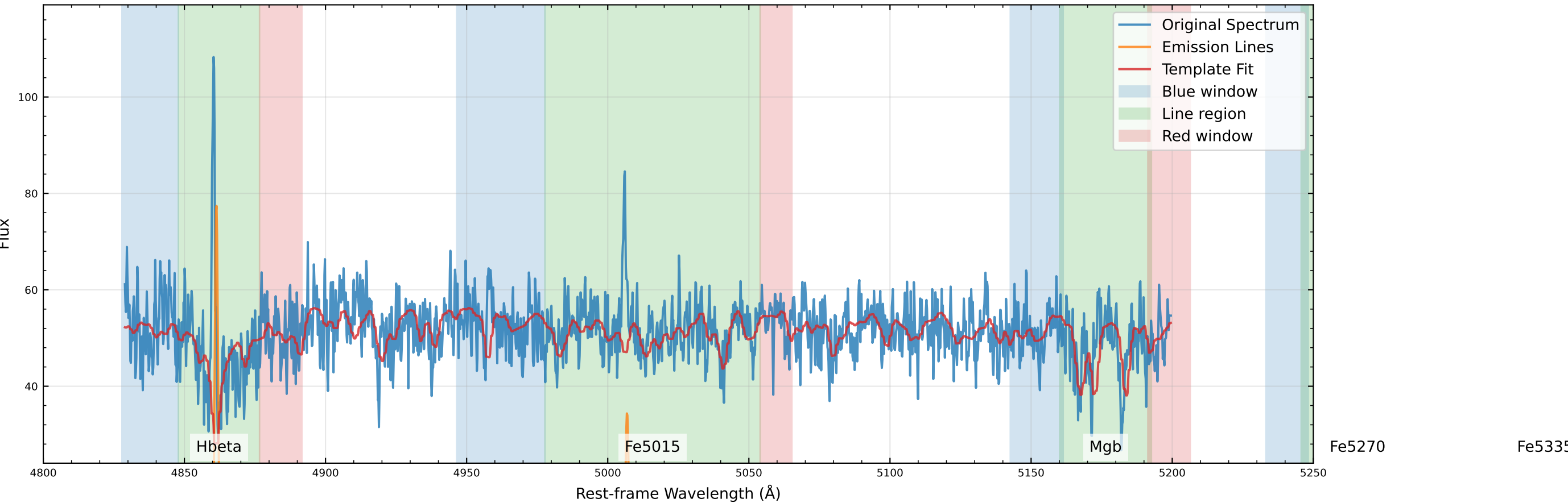
Original Data Comparison (v_star=-67.3 km/s, v_gas=-64.4 km/s)
