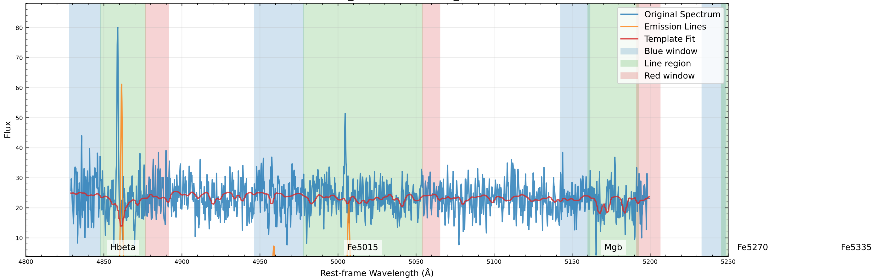
Original Data Comparison (v_star=-146.5 km/s, v_gas=-155.1 km/s)
