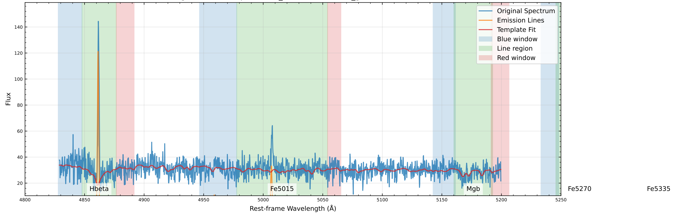
Original Data Comparison (v_star=40.8 km/s, v_gas=26.3 km/s)
