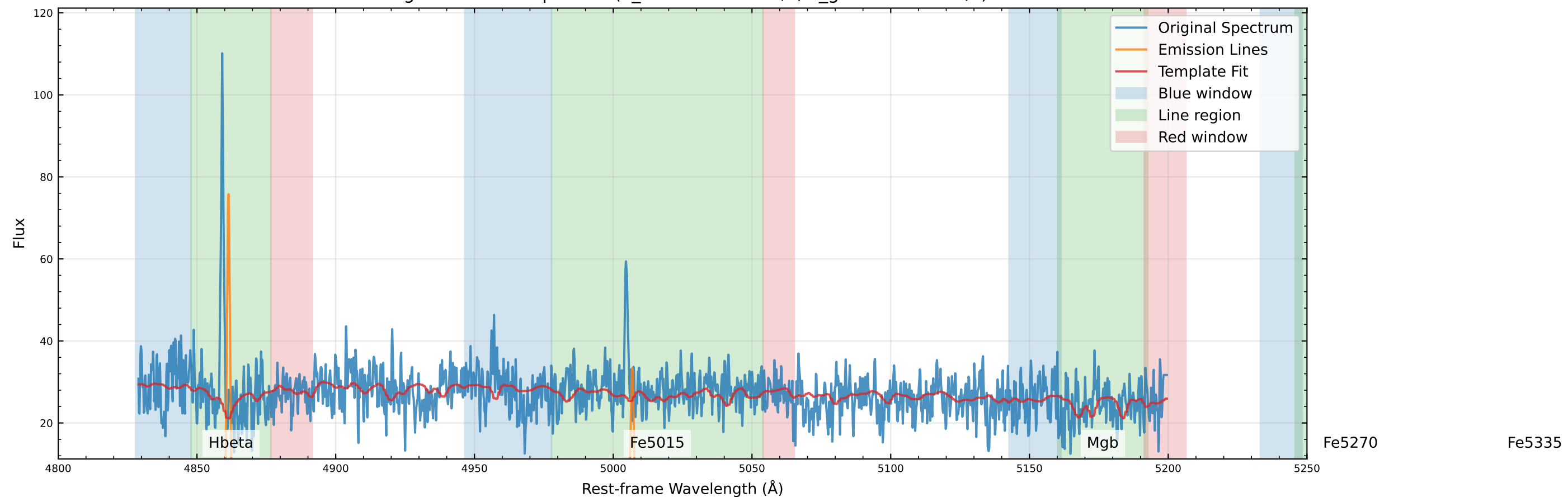
Original Data Comparison (v_star=-142.6 km/s, v_gas=-135.7 km/s)
