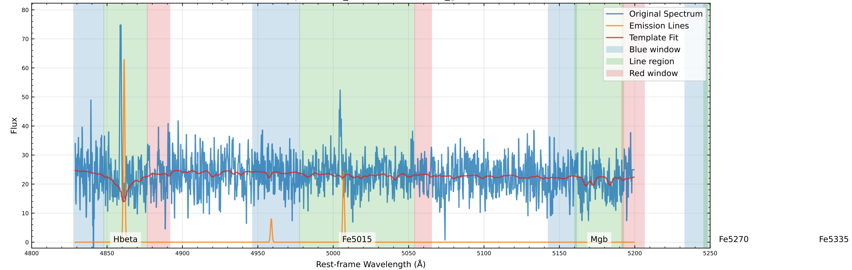
Original Data Comparison (v_star=-154.4 km/s, v_gas=-144.1 km/s)
