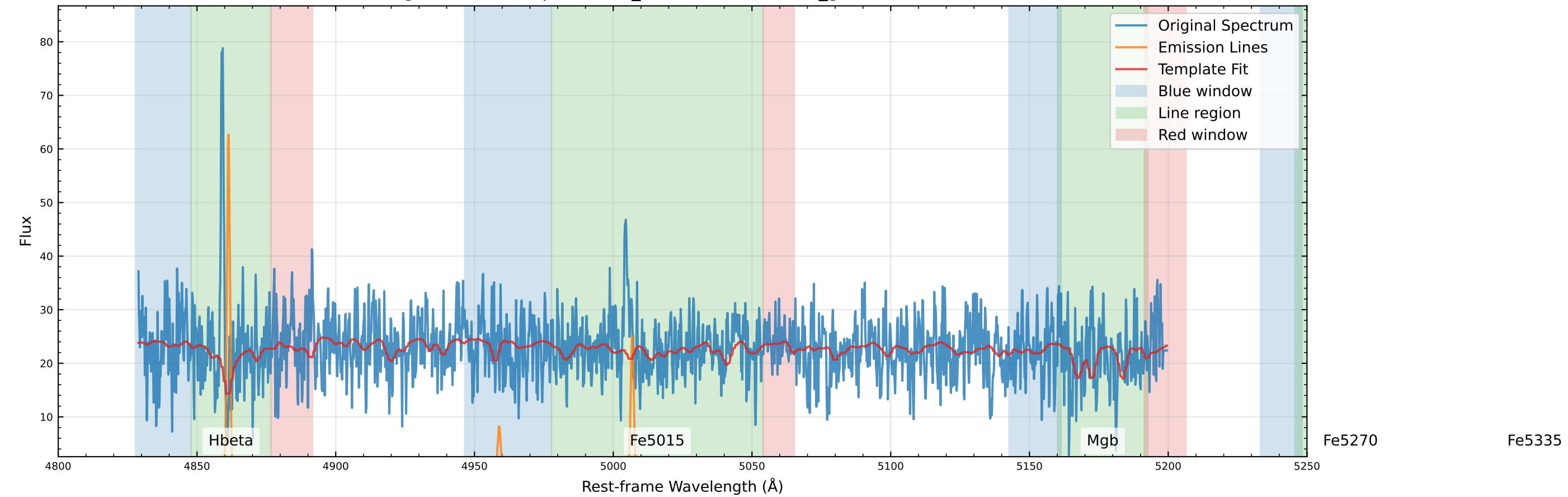
Original Data Comparison (v_star=-151.5 km/s, v_gas=-138.4 km/s)
