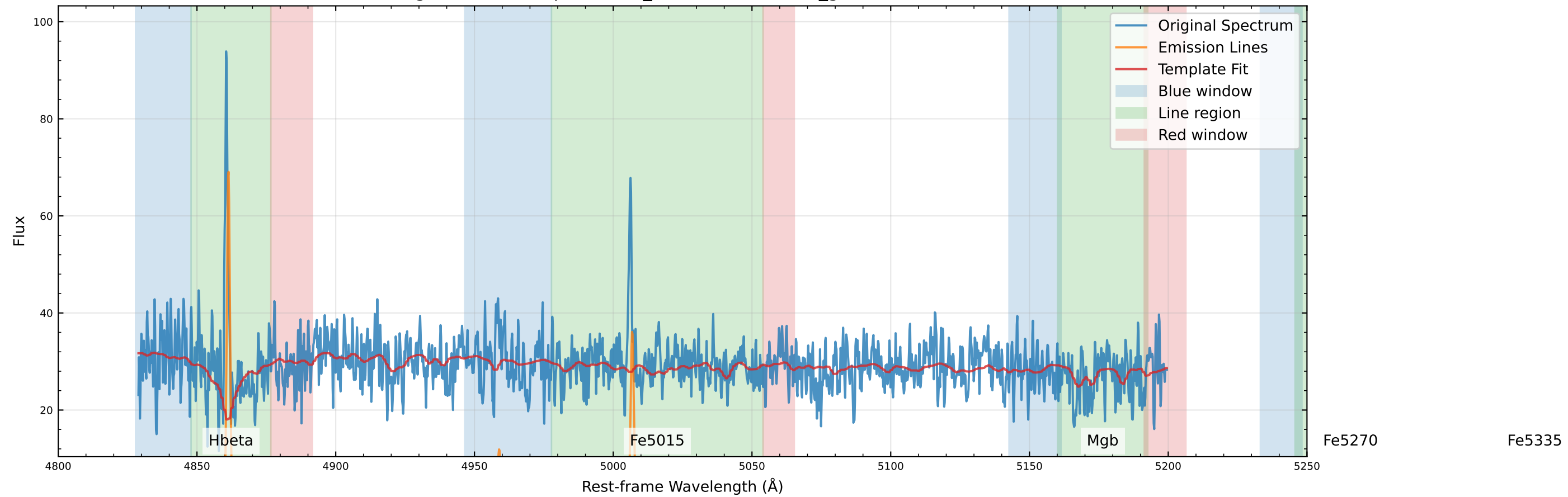
Original Data Comparison (v_star=-72.5 km/s, v_gas=-44.4 km/s)
