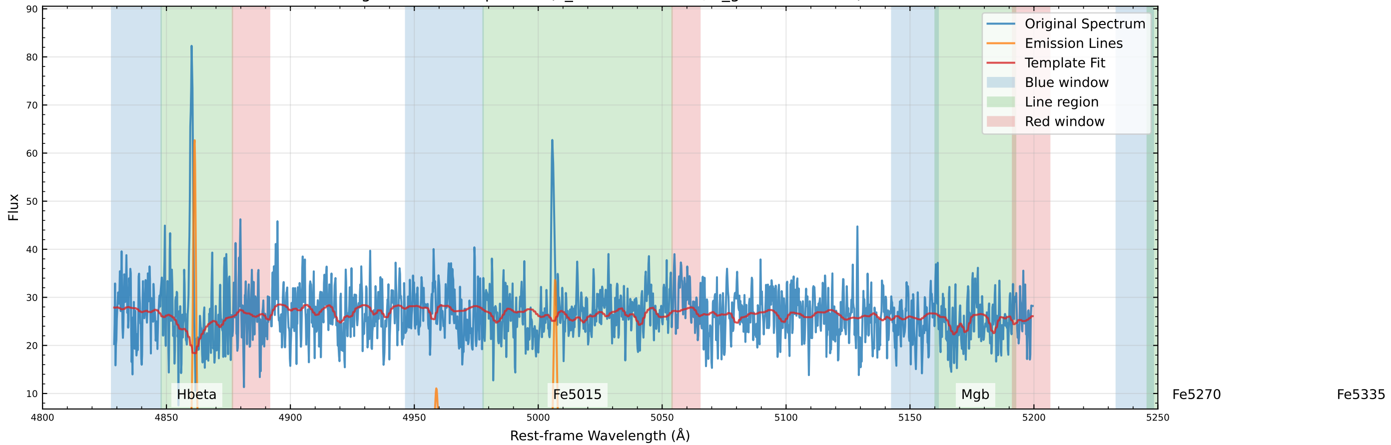
Original Data Comparison (v_star=-63.8 km/s, v_gas=-70.6 km/s)
