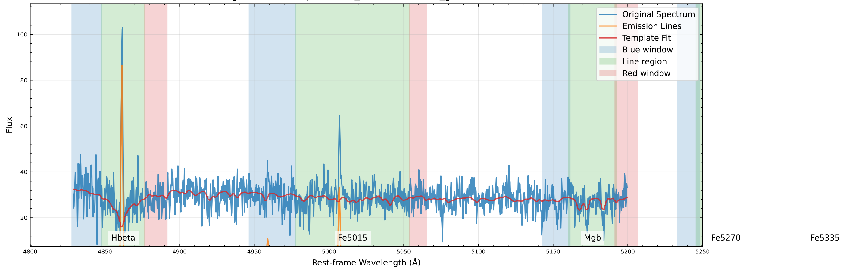
Original Data Comparison (v_star=6.8 km/s, v_gas=9.7 km/s)
