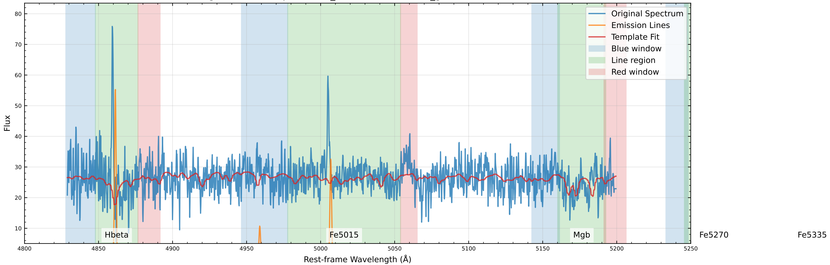
Original Data Comparison (v_star=-146.0 km/s, v_gas=-113.5 km/s)
