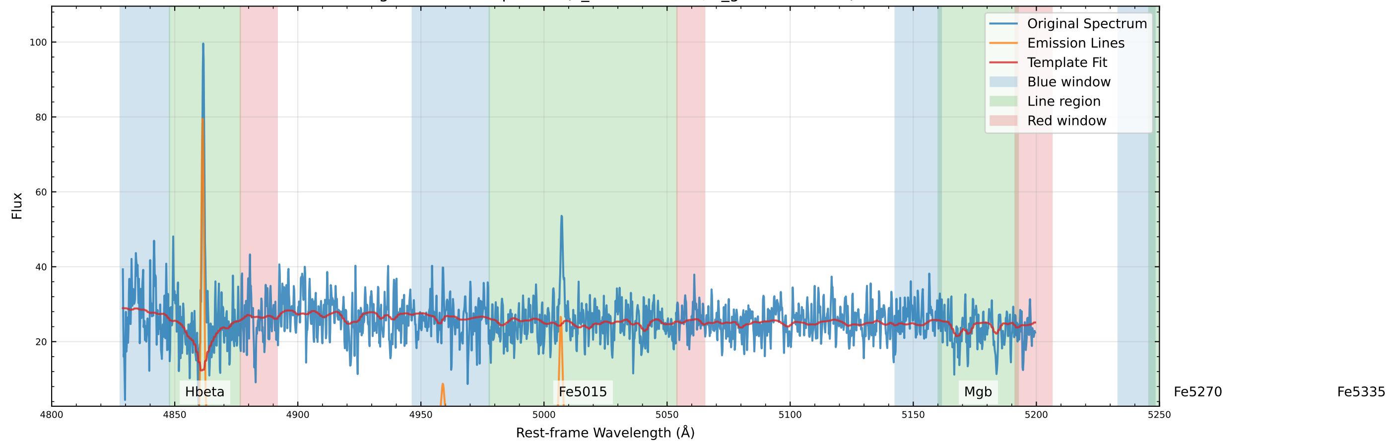
Original Data Comparison (v_star=4.3 km/s, v_gas=16.1 km/s)
