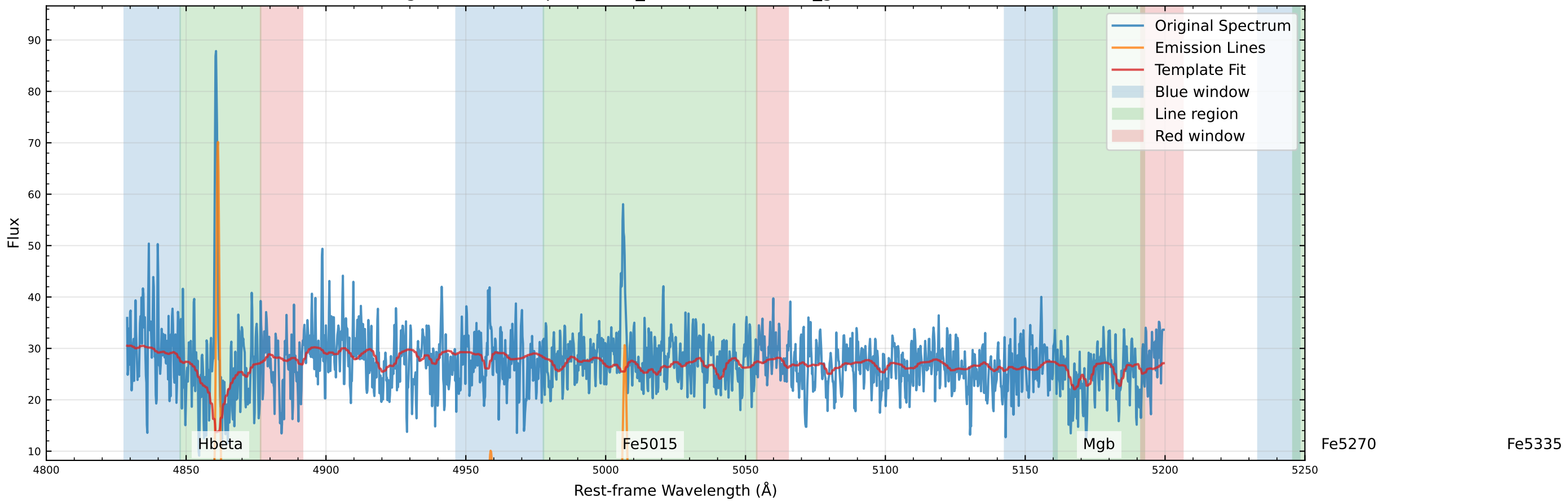
Original Data Comparison (v_star=-58.7 km/s, v_gas=-38.3 km/s)
