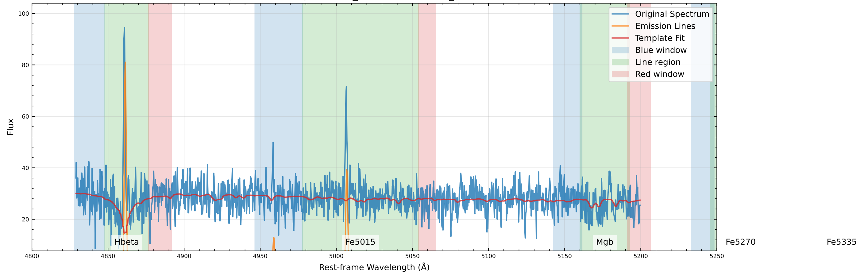
Original Data Comparison (v_star=-26.1 km/s, v_gas=-36.3 km/s)
