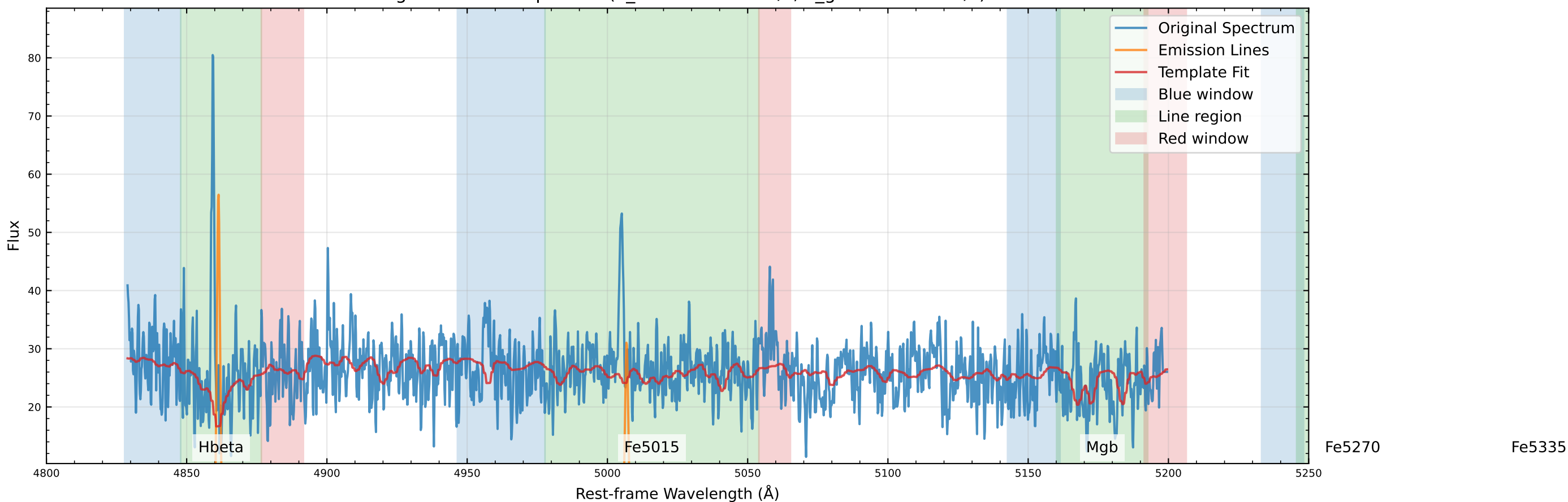
Original Data Comparison (v_star=-163.6 km/s, v_gas=-123.9 km/s)
