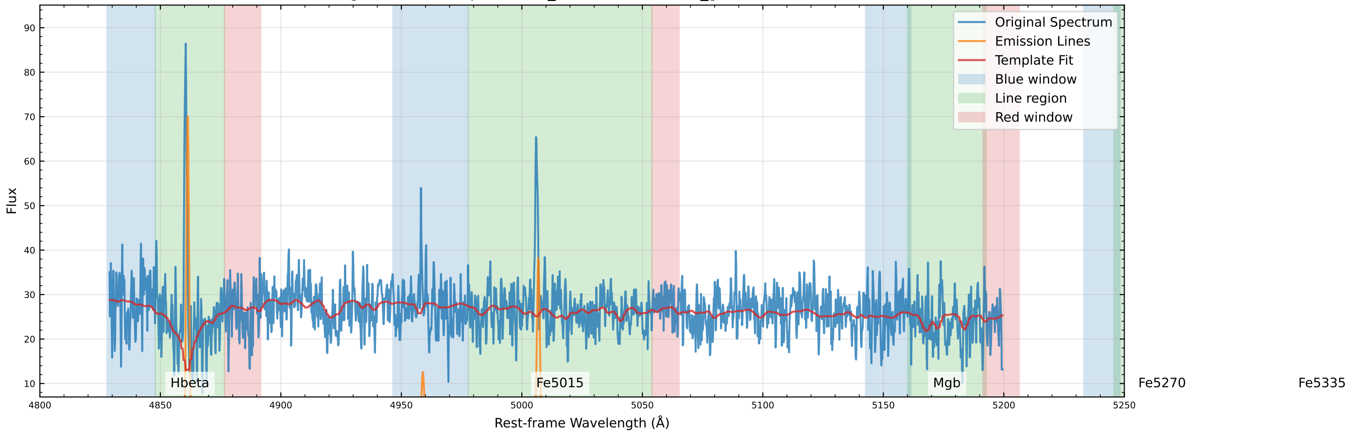
Original Data Comparison (v_star=-48.9 km/s, v_gas=-51.7 km/s)
