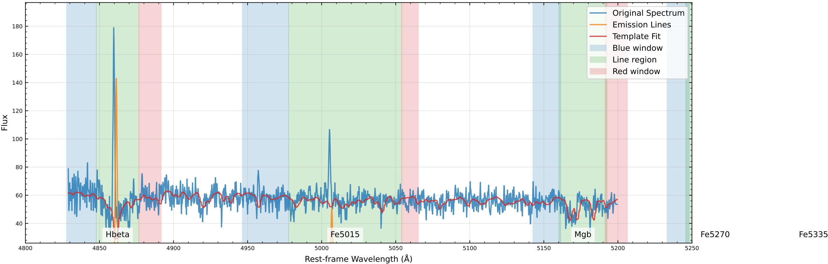
Original Data Comparison (v_star=-103.3 km/s, v_gas=-98.6 km/s)
