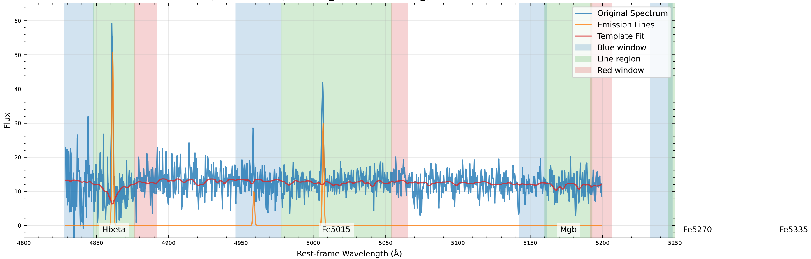
Original Data Comparison (v_star=-38.9 km/s, v_gas=-24.8 km/s)
