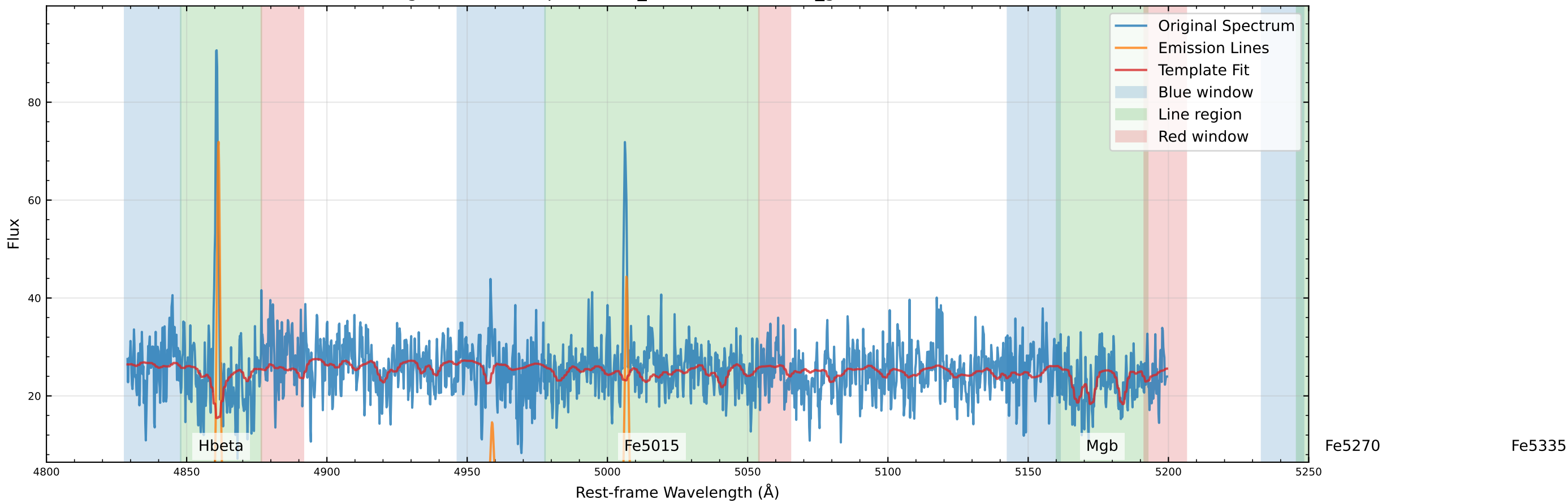
Original Data Comparison (v_star=-35.8 km/s, v_gas=-38.1 km/s)
