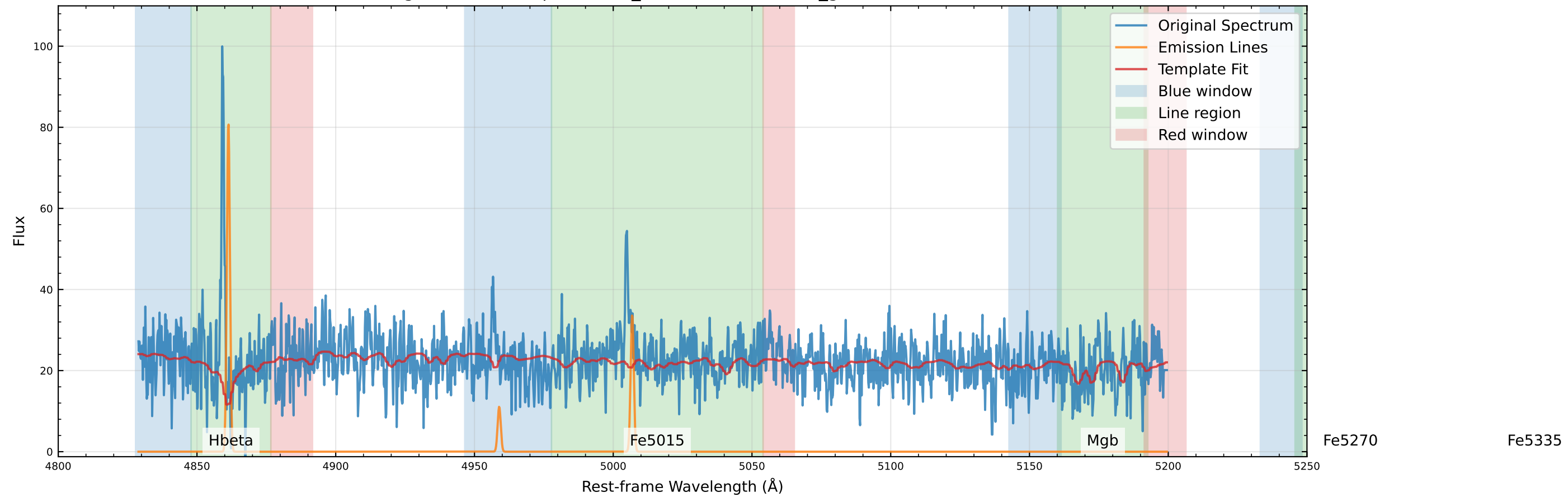
Original Data Comparison (v_star=-128.8 km/s, v_gas=-125.7 km/s)
