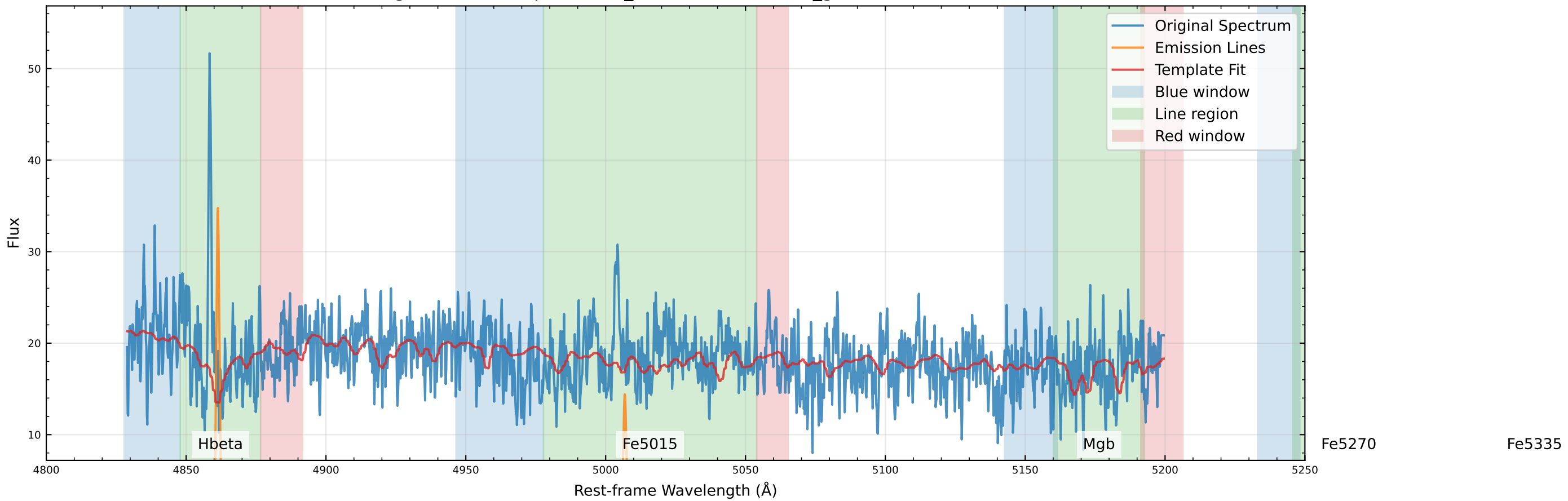
Original Data Comparison (v_star=-169.9 km/s, v_gas=-175.4 km/s)
