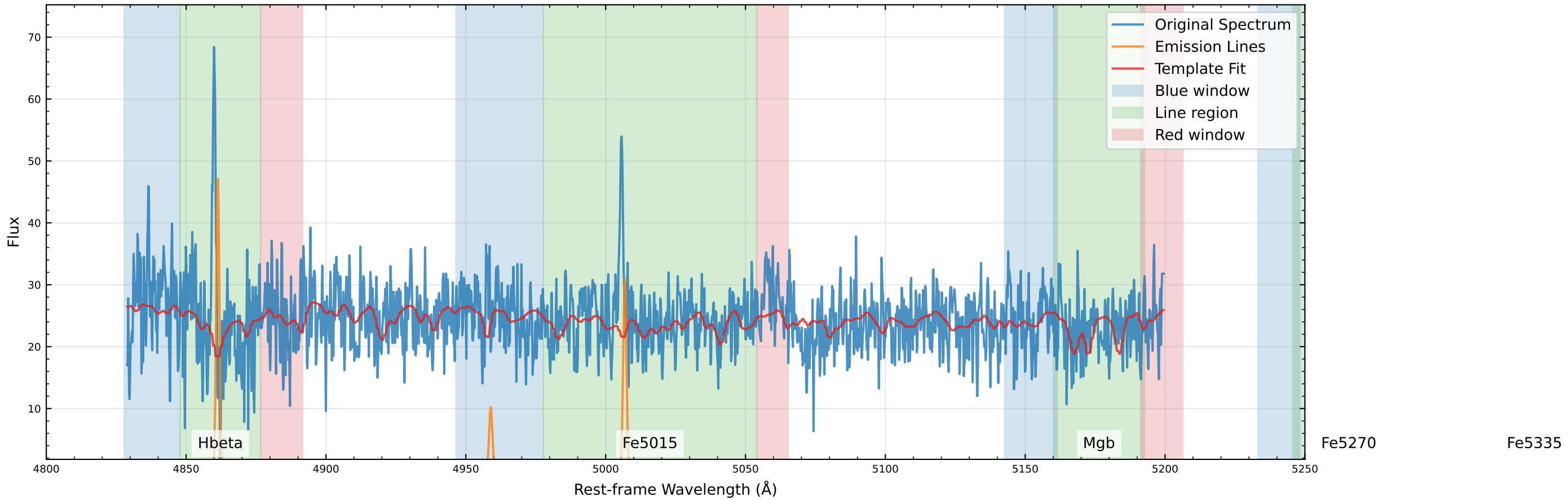
Original Data Comparison (v_star=-91.7 km/s, v_gas=-81.3 km/s)
