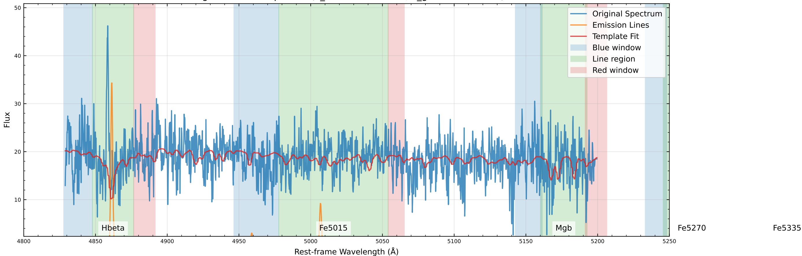
Original Data Comparison (v_star=-191.3 km/s, v_gas=-180.5 km/s)
