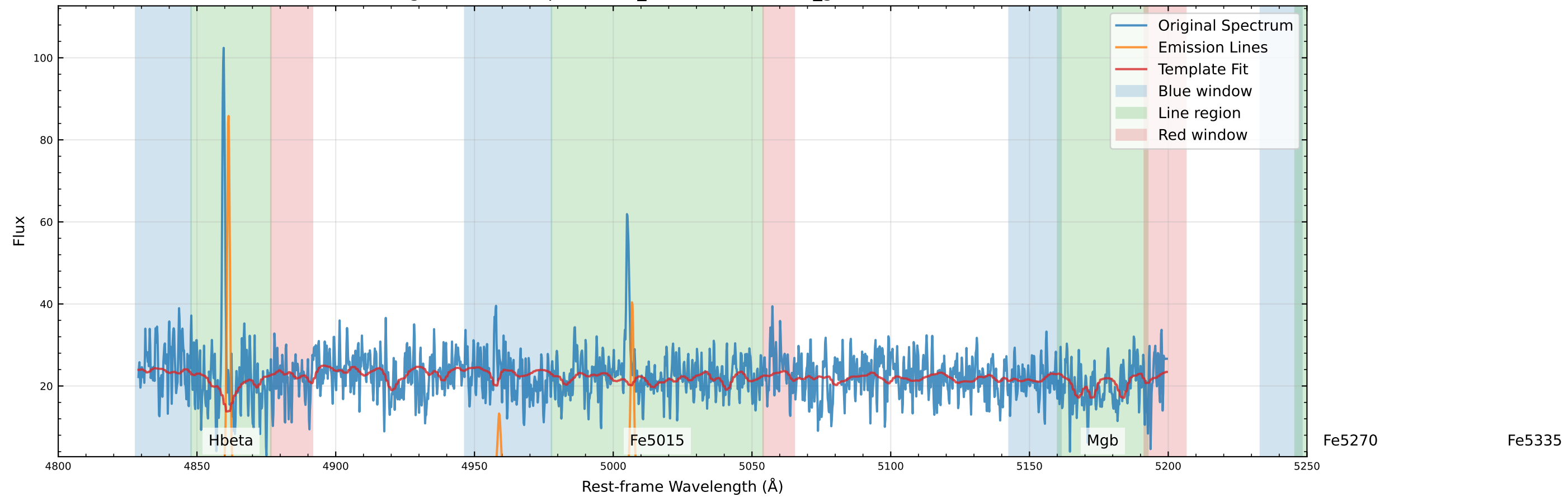
Original Data Comparison (v_star=-98.5 km/s, v_gas=-105.6 km/s)
